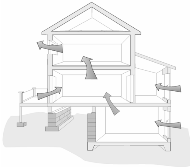
Figure 1-4 Stack Effect
