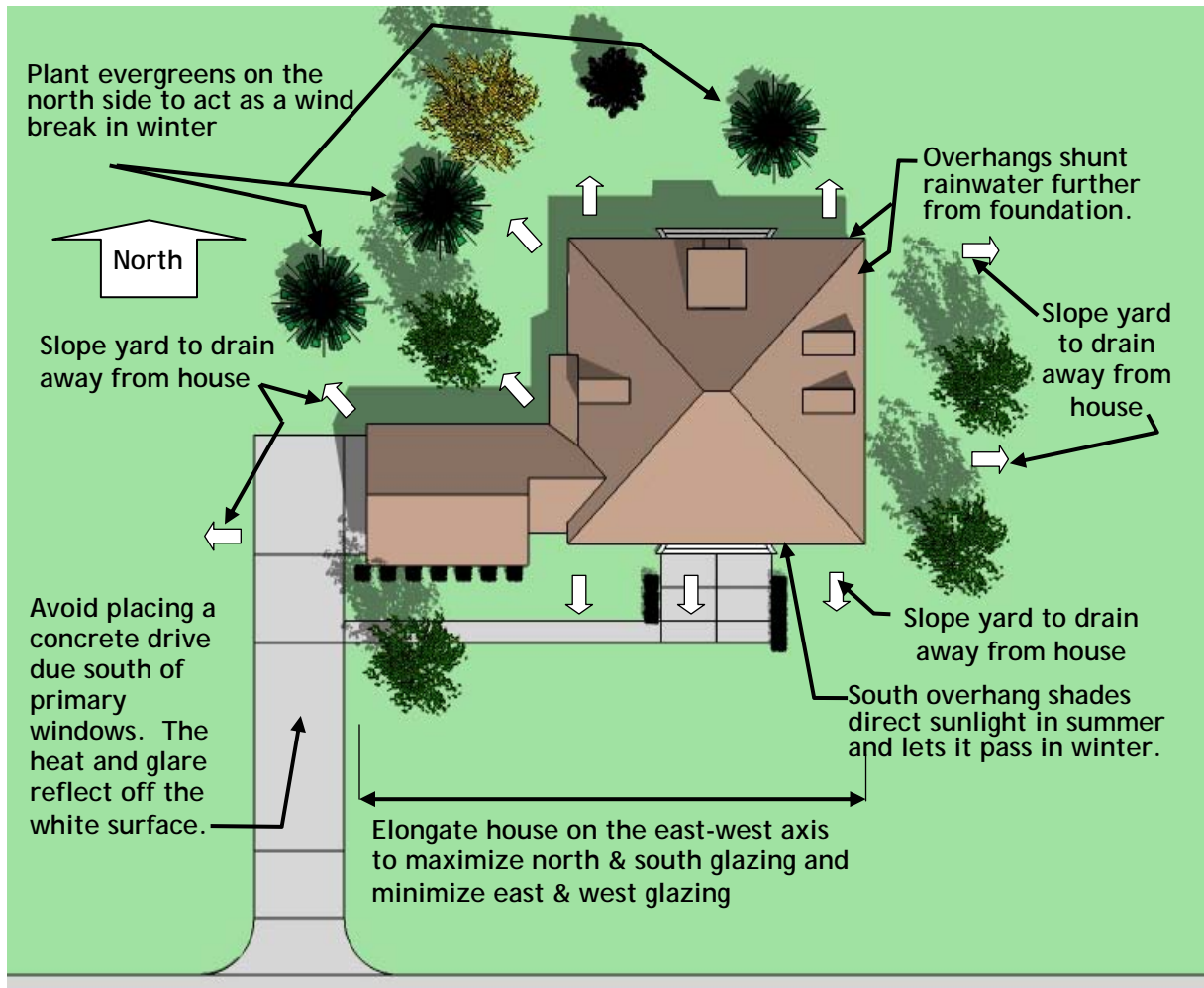
Figure 1-7 Site Planning
