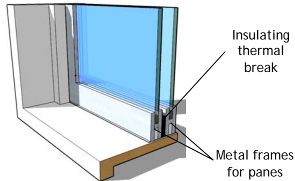
Figure 6-5 Metal Window with Thermal Break
